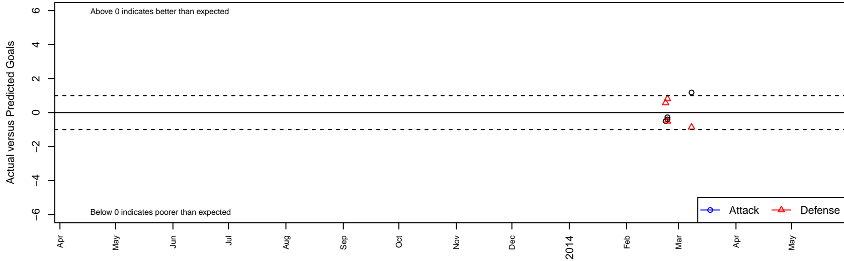
Carlsbad Wave FC Black B01 Dots are actual minus expected GF (blue circles) and GA (red triangles). Blue line is smoothed change in attack strength. Red is smoothed change in defense strength.
